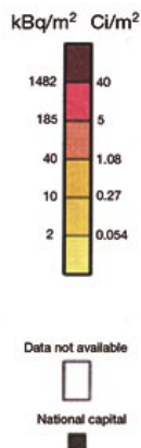
Distribution of ^{137}\text{Cs} following Chernobyl accident
