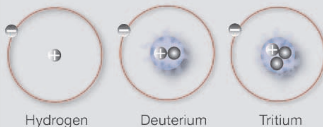
Isotopes of hydrogen
